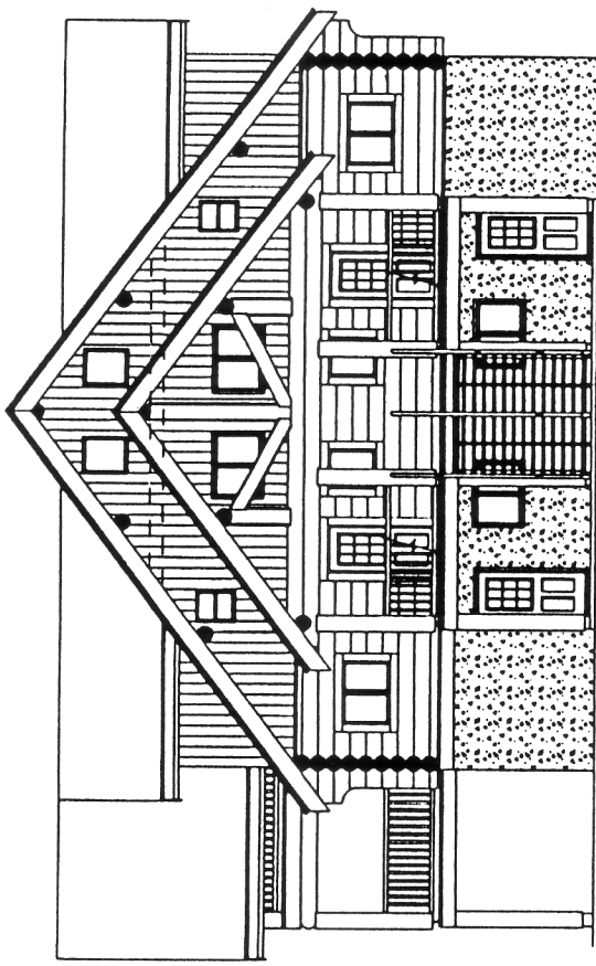
FRONT ELEVATION
