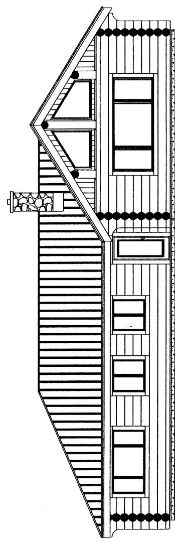
FRONT ELEVATION
