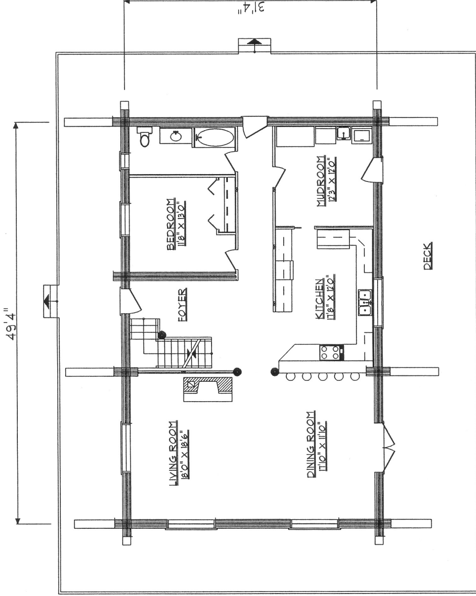
MAIN FLOOR PLAN 1600 $E
