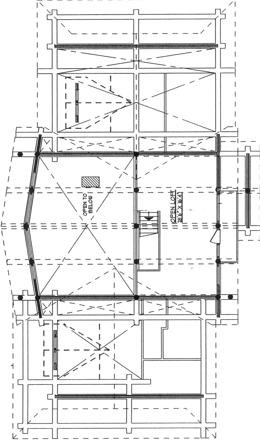
ROOF/LOFT FLOOR PLAN $25.9E
