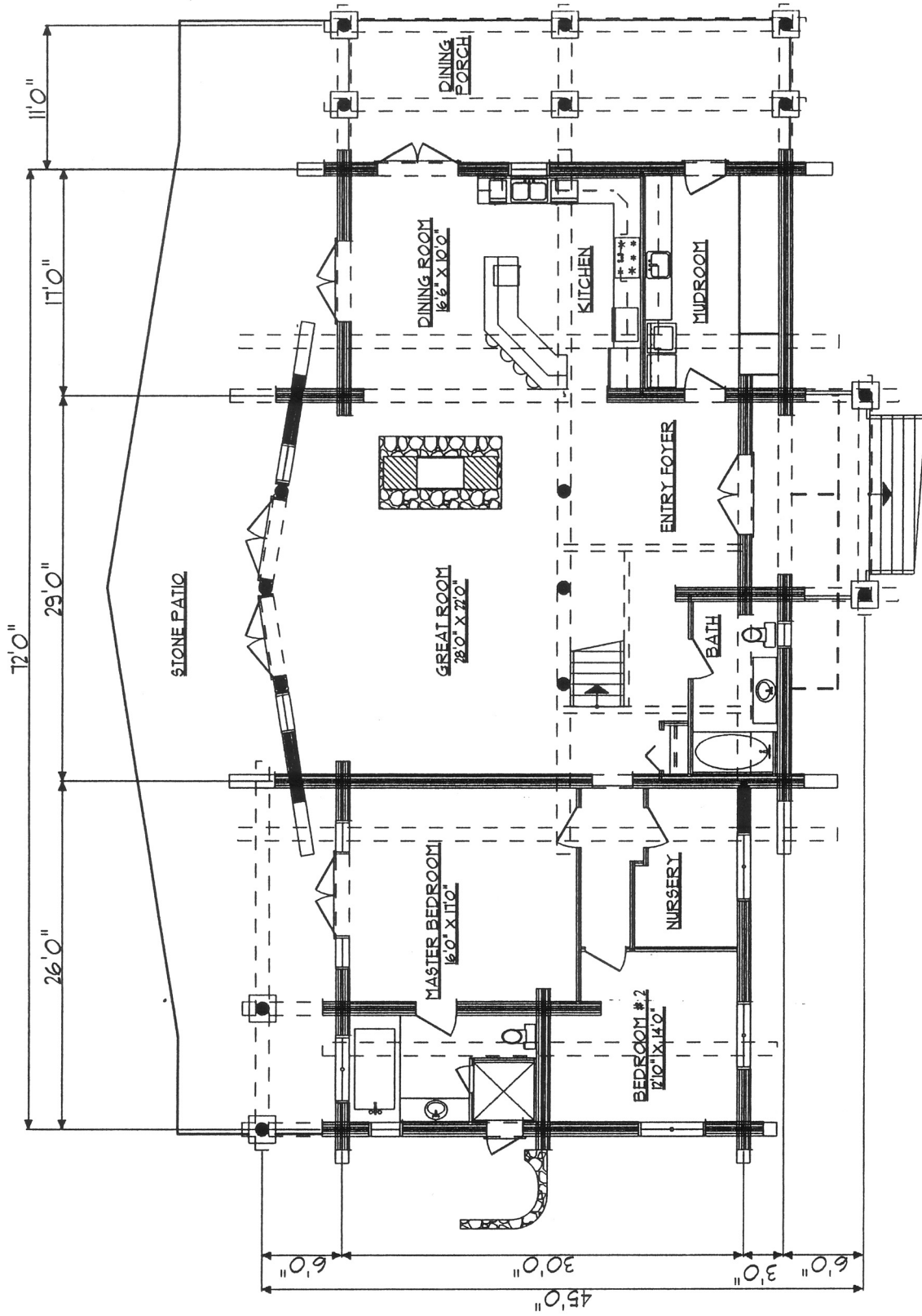
MAIN FLOOR PLAN HOUSE - 2500 SE
