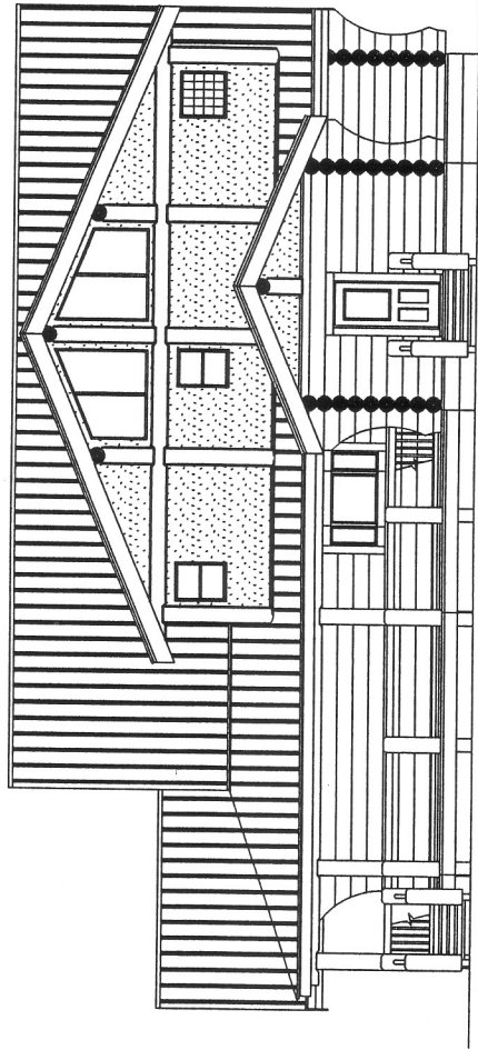
REAR ELEVATION
