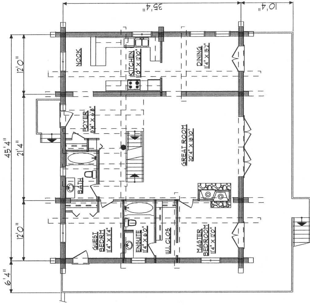
MAIN FLOOR PLAN 1656 SF
