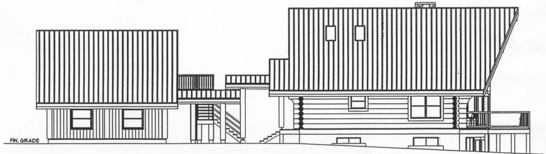
LEFT ELEVATION
