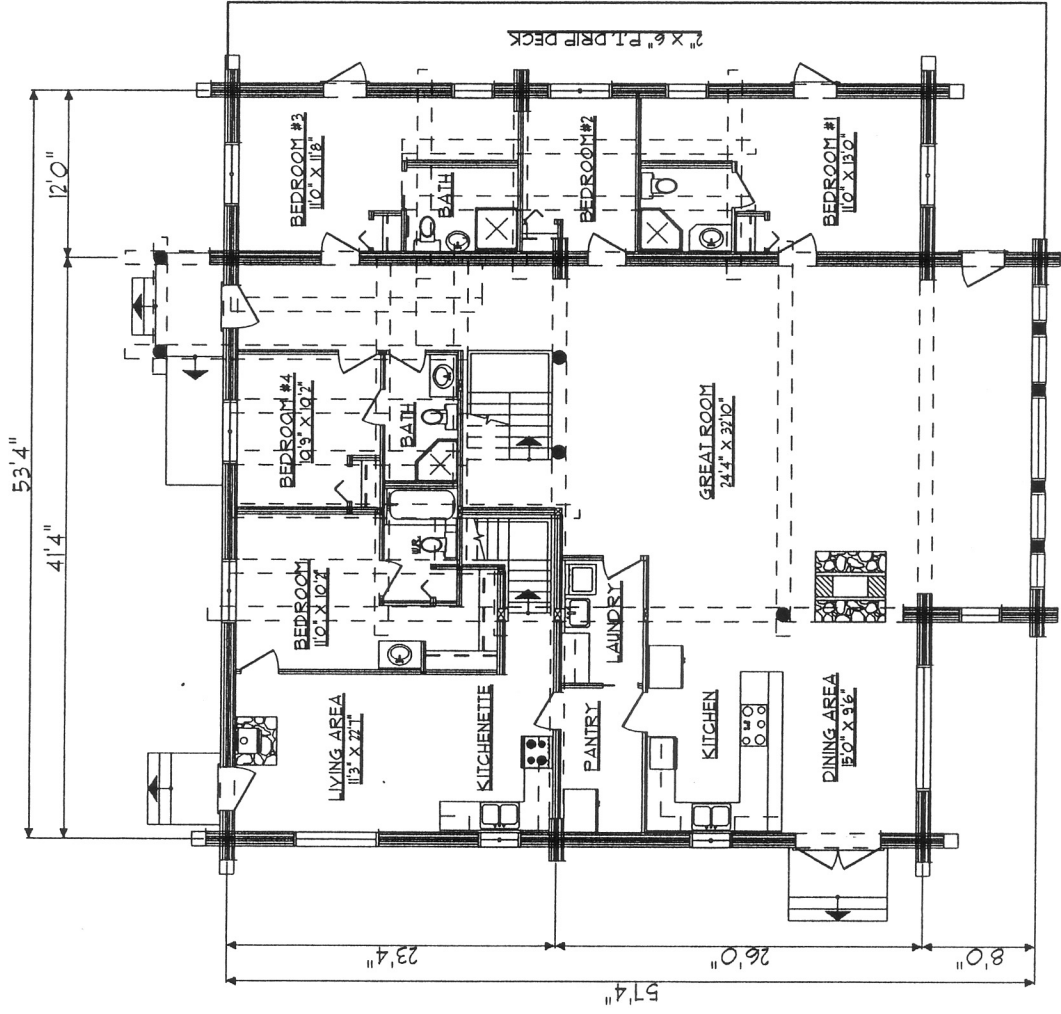
MAIN FLOOR PLAN 2902_SF
